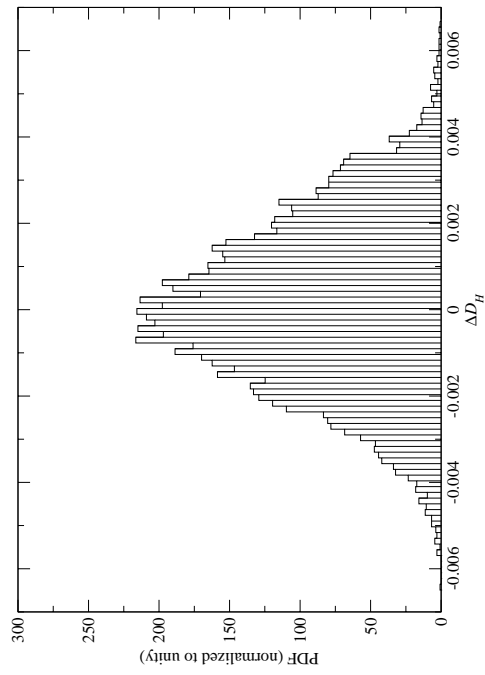
FIG. 3: Probability distribution function (PDF) for finding an estimate for the fractal dimension D_H that deviates by amount \Delta D_H in the q = 4 case. Histogram was obtained by sampling 10000 synthesized data sets.
