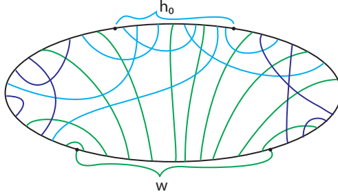
FIGURE 5. Reducing diagram indicating subword h_0 . Light blue and dark blue arcs emanate from h .
