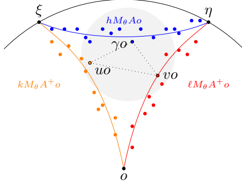
FIGURE 5. The dotted triangle is of diameter less than C and the gray ball has radius R .
